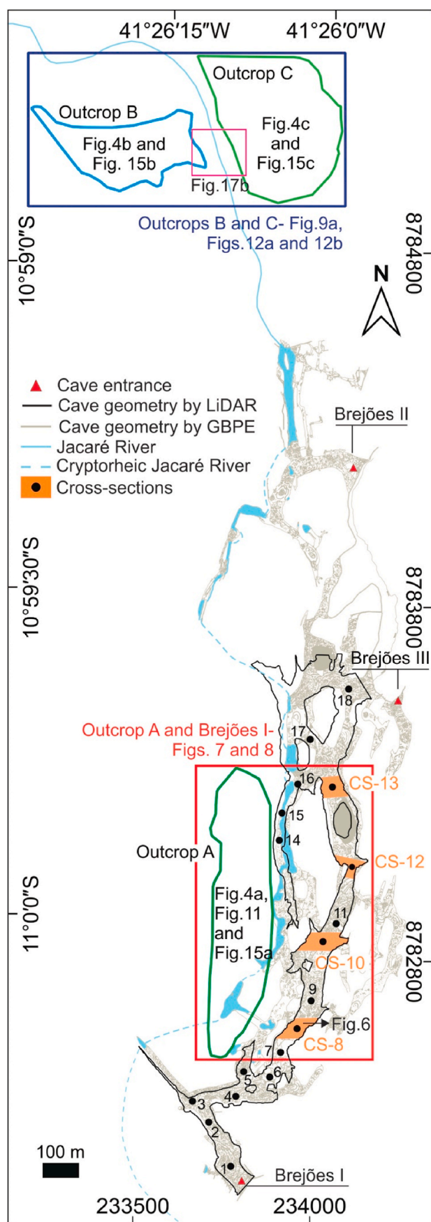
Fig. 2. General view of the study area locating all outcrops and caves. Outcrops A (dark green polygon), B (light blue polygon), and C (light green polygon) were used to perform the statistical characterization of the fracture networks. The dark blue rectangle encompasses outcrops B and C, which were also used to compare persistence variation along an anticline coinciding with the Jacaré river valley. The pink rectangle represents the area of the block diagram used to show the actual configuration of Brejões canyon (Fig. 17b). The red rectangle encompasses sectors of Outcrop A, and the contiguous subsurface caves (filled orange polygons), which is used to compare fracture networks in corridors and caves. The black dots show the cave cross-sections located along the Brejões I System. This figure is presented in geographic and UTM coordinate systems to facilitate localization at different scales. Cave mapping done by GBPE ("Grupo Bambuí de Pesquisas Espeleológicas") ( https://bambuiespeleo.wordpress.com/ ). (For interpretation of the references to colour in this figure legend, the reader is referred to the Web version of this article.)
