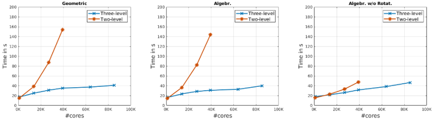
Fig. 4: Weak parallel scalability for the three- and two-level method with a reduced dimensional coarse space; see Table 1 for the data.
