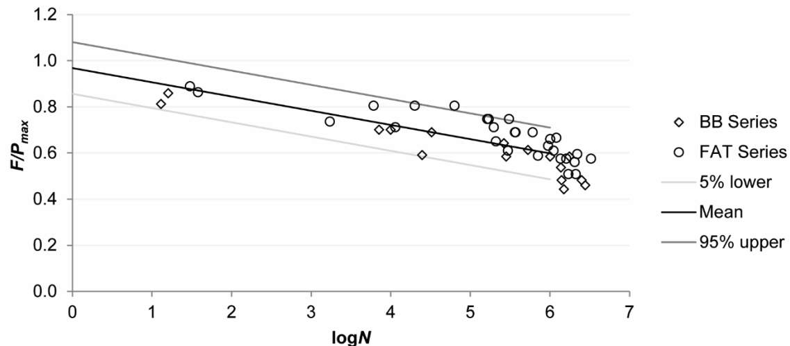
Figure 6. Relation between the number of cycles N and the applied load ratio F/P_{\max} in all the fatigue experiments, adapted from Reference [37]. Reprinted with permission. This figure was originally published in Vol. 116 of the ACI Structural Journal.
