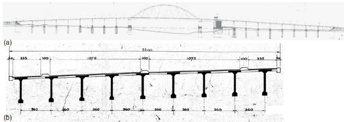
Figure 1. Van Brienenoord Bridge: (a) sketch of the elevation of the entire bridge structure, showing the approach slabs, as well as the steel arch; (b) cross-section of the slab-between-girder approach bridge. Dimensions in cm.
