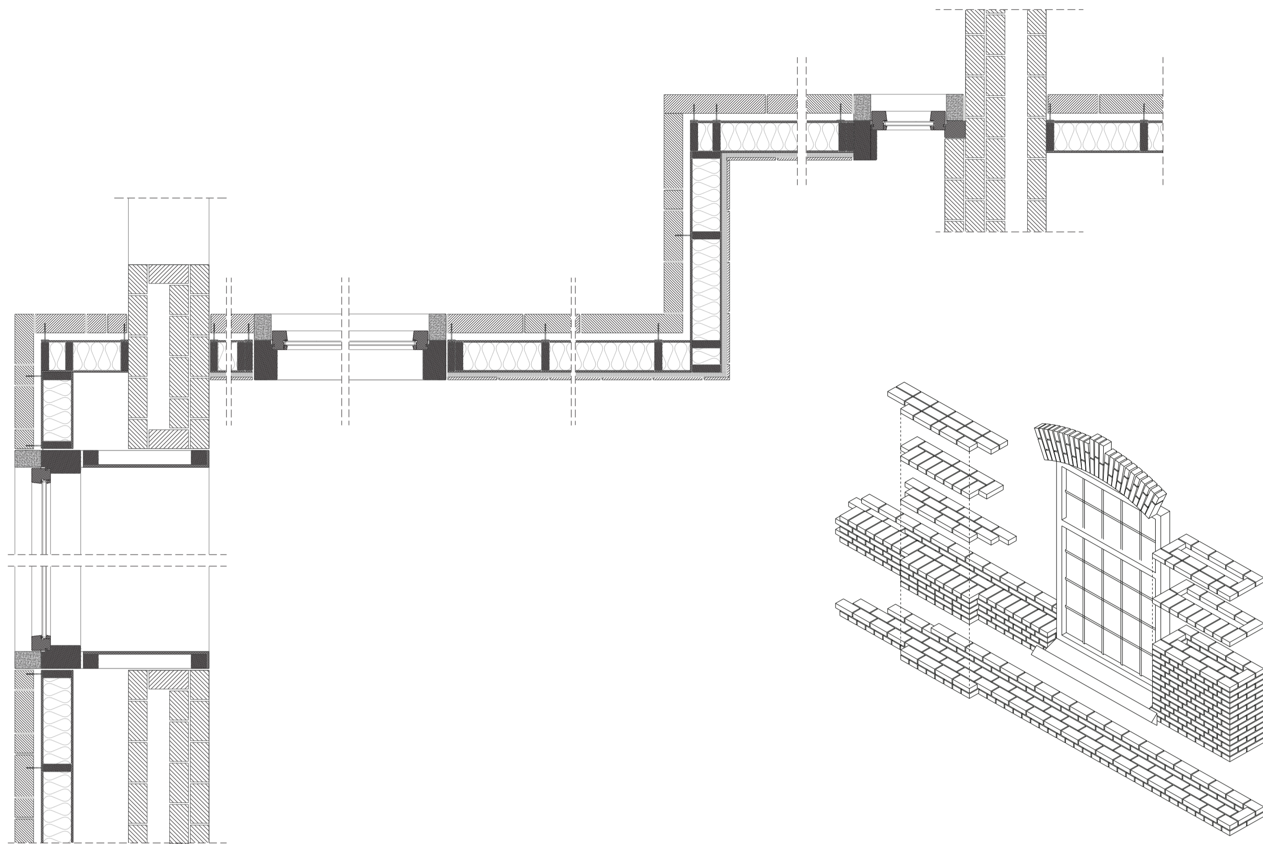
Horizontal details scale 1:20
