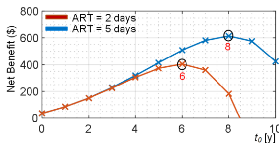
Fig. 11. Average Repair Time ( ART ) impact on the net benefit due to the delaying the converter replacement by t_0 - IC = 0.2 $/kWh, AMC = 250 $.
