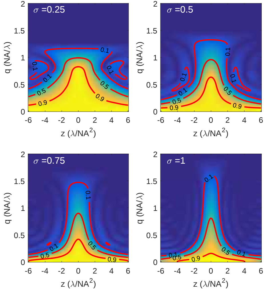
Figure 5: Numerically computed absolute value of the FT of the through-focus transfer function \left| \hat{Q}(\vec{q}) \right| for different values of the partial coherence factor \sigma .
