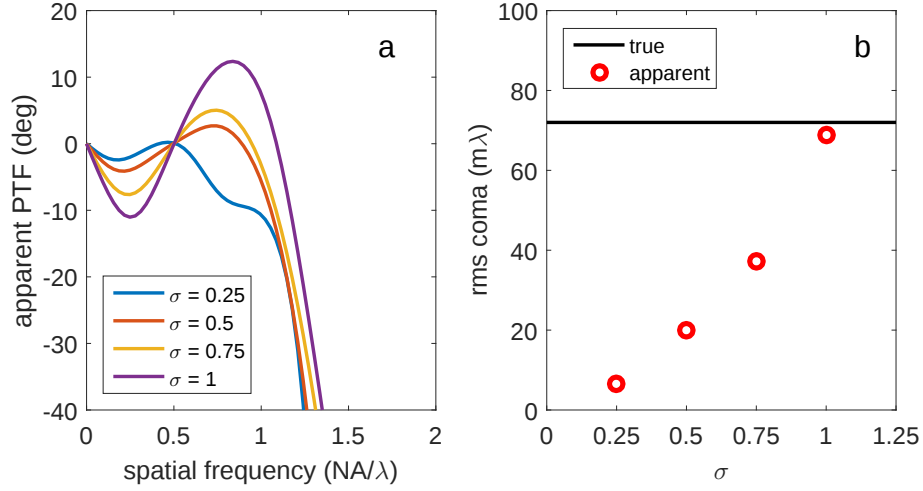
Figure 9: (a) Simulated PTF with 72 mλ rms coma for different values of the partial coherence factor \sigma values as a function of the spatial frequency. (b) The estimated coma based on the method of Ref. [16] as a function of \sigma .
