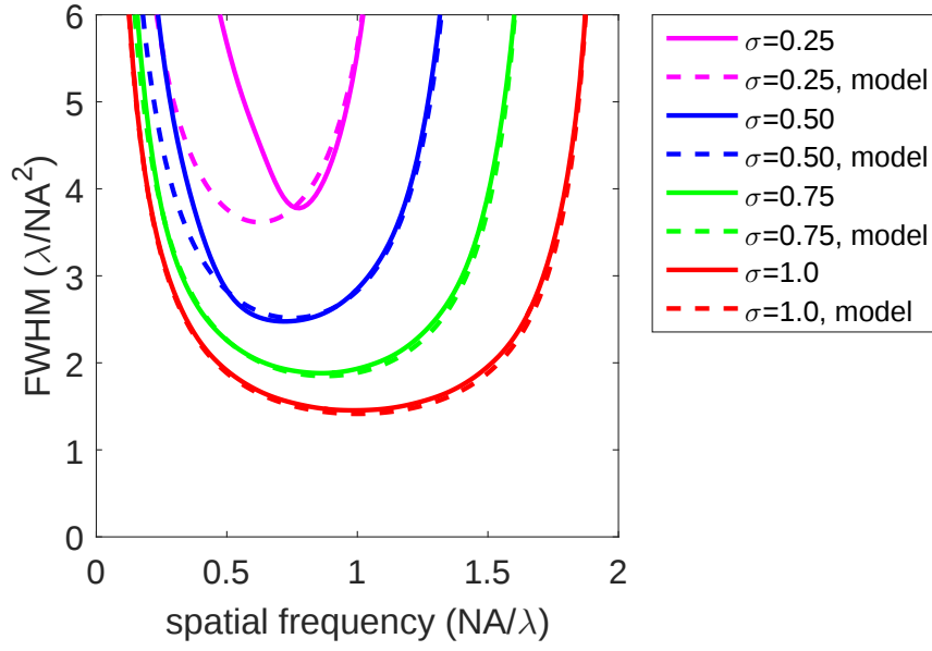
Figure 6: Numerically computed FWHM of the through-focus transfer function \left| \hat{Q}(\vec{q}) \right| as a function of the spatial frequency for different values of the partial coherence factor \sigma and the corresponding predictions of Eq. (27) with \beta = \sqrt{2} .
