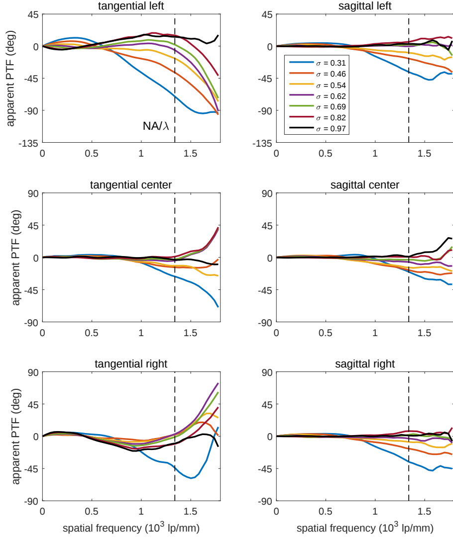
Figure 15: Measured in-focus apparent PTF curves for the green channel and for tangentially and sagittally oriented edges for the left (-0.5 mm), center and right (+0.5 mm) of the FOV for different values of the partial coherence factor \sigma . The dashed lines indicates the spatial frequency NA/\lambda .
