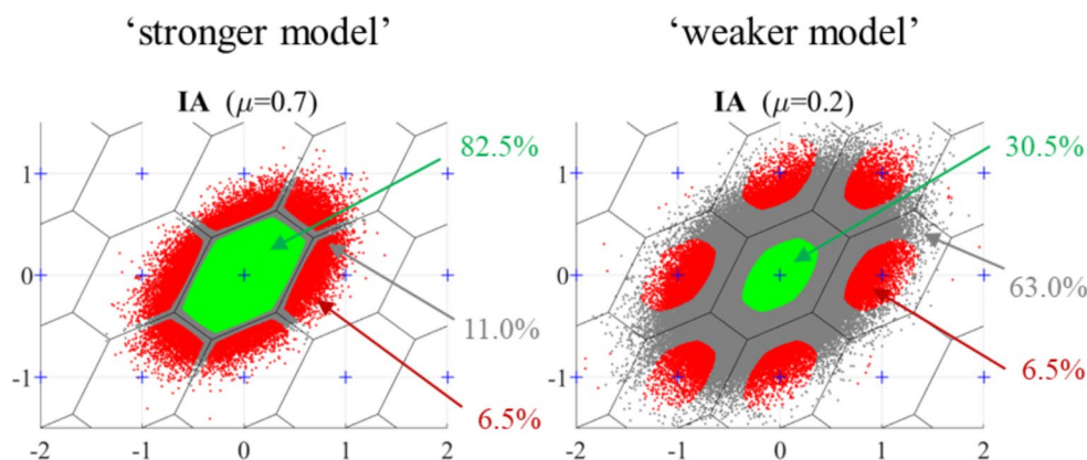
Fig. 6 A comparison between a stronger and a weaker model is given using two different ratio tests, respectively for \mu = 0.7 and \mu = 0.2 . Three regions can be observed, related to values of Success Rate (green), Failure Rate (red) and Undecided Rate (grey)
