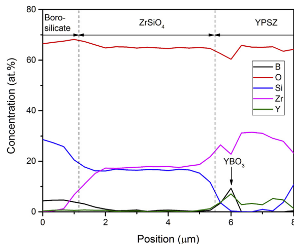
Fig. 6. Chemical composition profile across the YPSZ – \text{MoSi}_2(\text{B}) interdiffusion couple after annealing at 1200 °C in laboratory air for 96 h, as obtained with EPMA. Error less than 0.5 at.% for each element.
