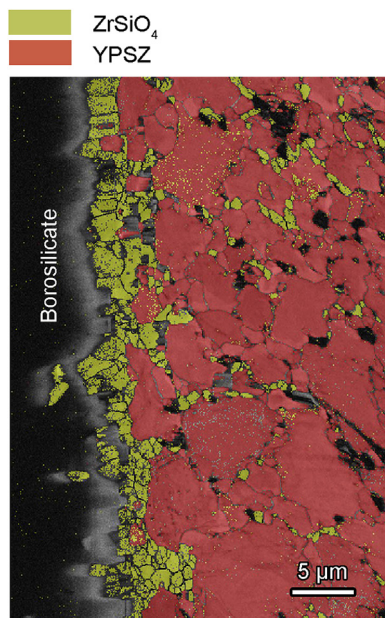
Fig. 7. Phase map of YPSZ-MoSi 2 (B) interdiffusion couple after annealing at 1200 °C in laboratory air for 96 h, showing the ZrSiO 4 formation at the YPSZ – SiO 2 + 5 at.% B interface and along grain boundaries of YPSZ as obtained by SEM –EBSD of a cross section.
