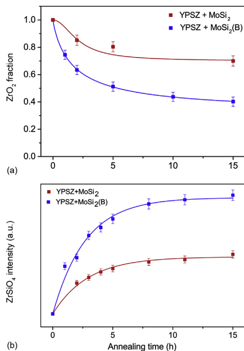
Fig. 4. Kinetic curves of (a) \text{ZrO}_2 consumption and (b) \text{ZrSiO}_4 formation in mixtures of YPSZ – \text{MoSi}_2 (red) and YPSZ – \text{MoSi}_2(\text{B}) (blue) during annealing at 1100 °C in laboratory air as obtained from (ex situ) XRD analysis considering the (112) and (020) \text{ZrO}_2 and (200) \text{ZrSiO}_4 diffraction lines. Error corresponds to 3 times the standard deviation of the number of photons counted (Poissonian distribution). (For interpretation of the references to colour in this figure legend, the reader is referred to the Web version of this article.)
