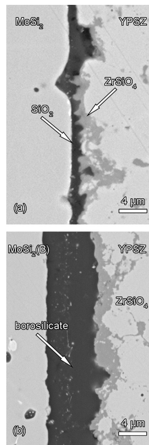
Fig. 5. SEM backscattered electron images of cross-section of (a) YPSZ – \text{MoSi}_2 and (b) YPSZ – \text{MoSi}_2(\text{B}) interdiffusion couples after annealing for 96 h at 1100 °C in laboratory air. A silica layer (a) or borosilicate layer (b) is developed due to oxidation of \text{MoSi}_2 and \text{MoSi}_2(\text{B}) , respectively. The very small bright phase at the edge of \text{MoSi}_2 and \text{MoSi}_2(\text{B}) belongs to \text{Mo}_5\text{Si}_3 . In between the silica or borosilicate layer and the YPSZ, zircon ( \text{ZrSiO}_4 ) is formed.
