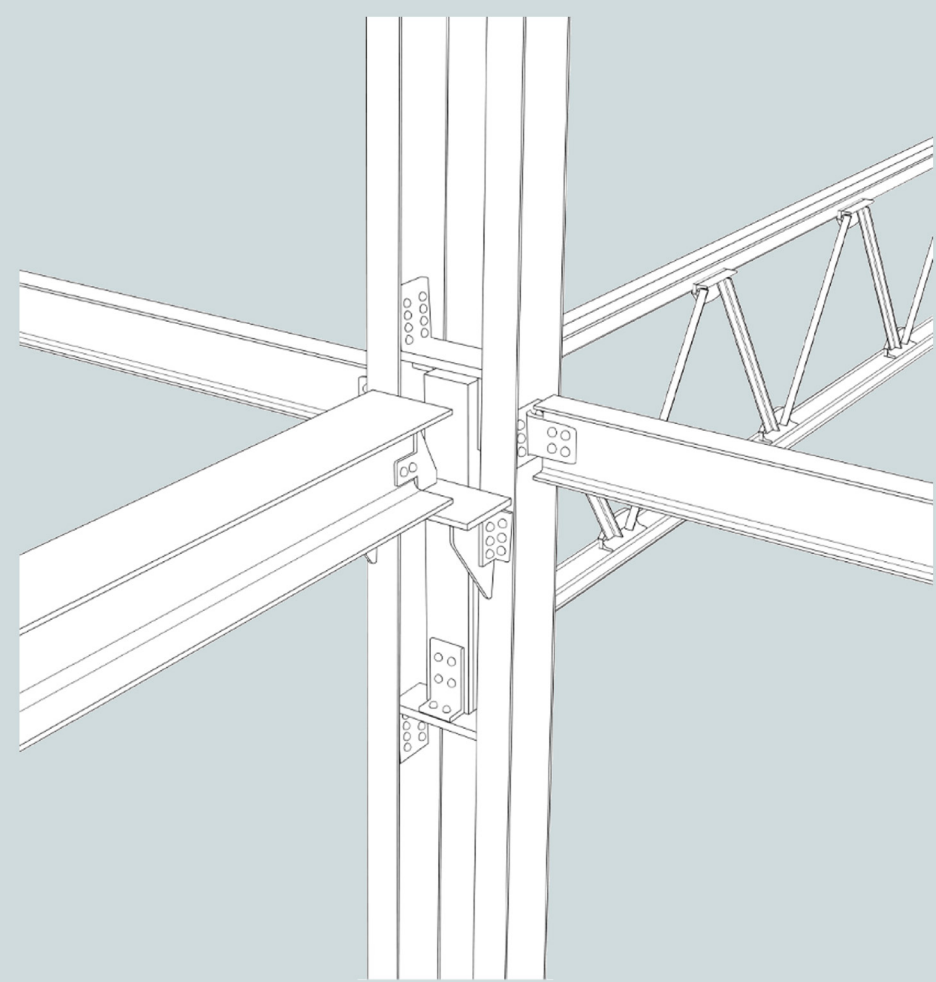
CONNECTION HEA 260 COLUMN - ANGLED IPE 260 COLUMNS 1TH FLOOR ONLY
