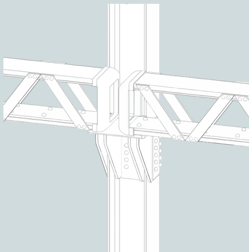
CONNECTION REUSED TRUSS - COLUMN - PRIMARY / SECONDARY BEAMS 2ND, 3RD, 4TH, 5TH FLOOR
