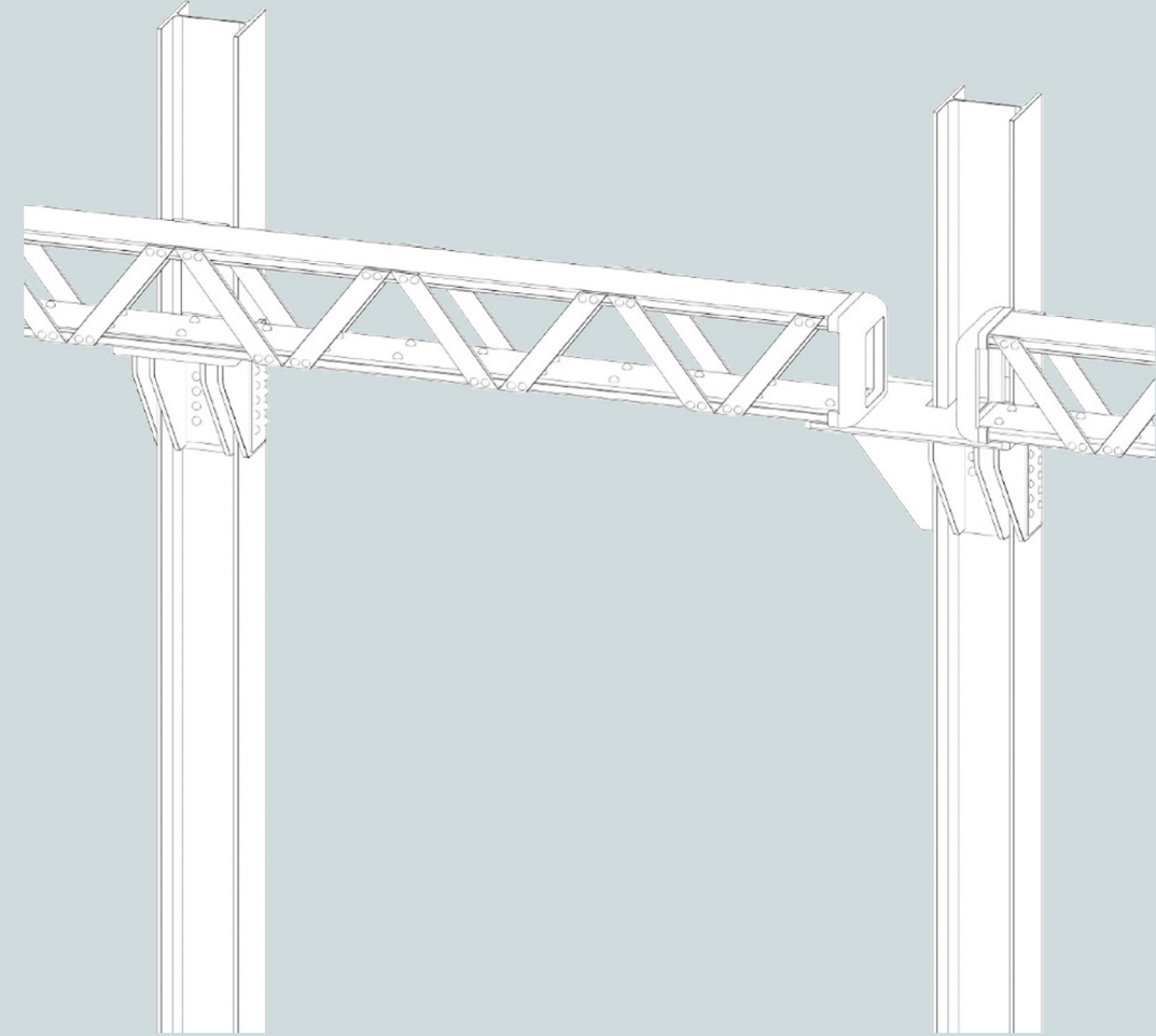
CONNECTION REUSED TRUSS - COLUMN GROUND FLOOR
