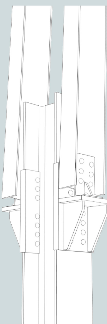
CONNECTION HEA 260 COLUMN - ANGLED IPE 260 COLUMNS 1TH FLOOR ONLY
