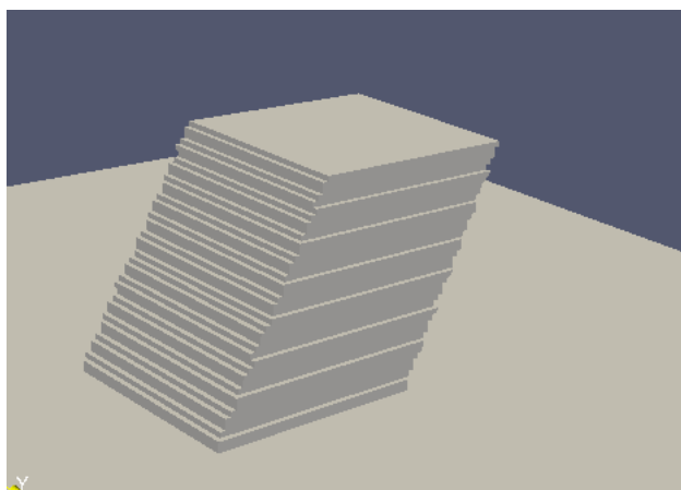
Fig. 12. Shifted block showing the cause of striped walls
