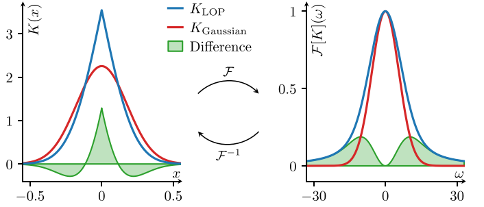
Fig. 3. Comparison of LOP and Gaussian kernels in spatial and frequency domain. Filtering with the LOP kernel K_{LOP} better preserves higher frequency information.
