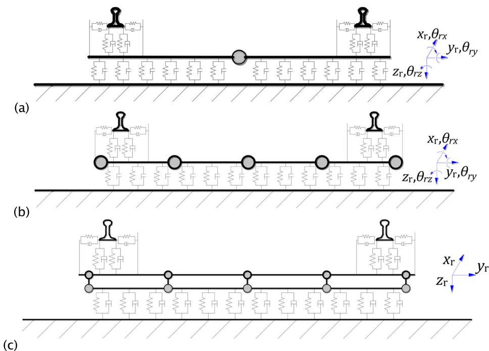
Figure 2. Ballast track model for different finite elemental sleepers, end view. (a. rigid body sleeper; b. elastic-beam element sleeper; c. solid element sleeper).
