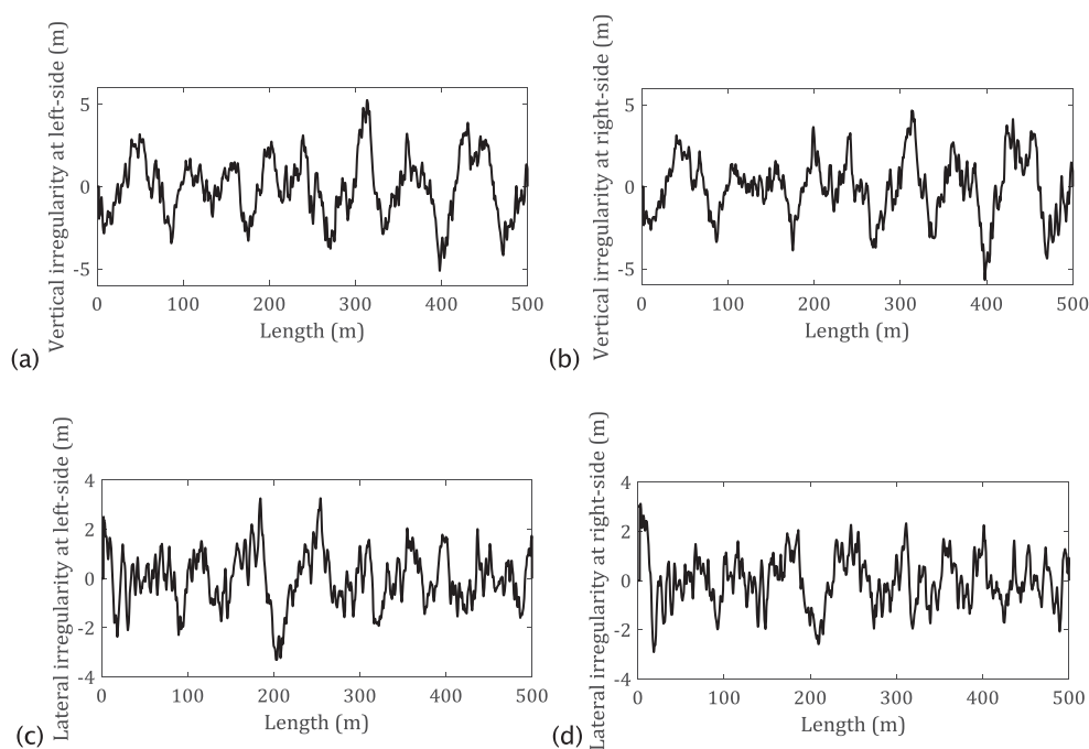
Figure 9. Track irregularity excitation (a. vertical irregularities at the left-side of the rail; b. vertical irregularities at the right-side of the rail; c. lateral irregularities at the left-side of the rail; d. lateral irregularities at the right-side of the rail).
