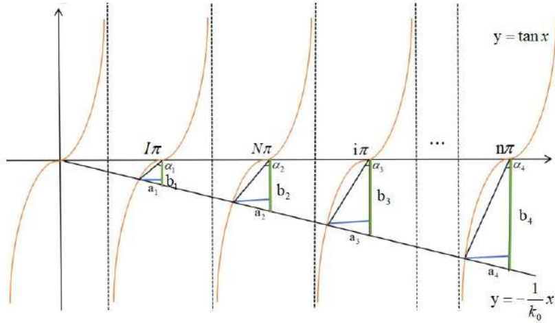
Figure 2.8: Graphical comparisons of eigenvalues for k_0 = \infty and 0 < k_0 < \infty with I+N+i=n .
