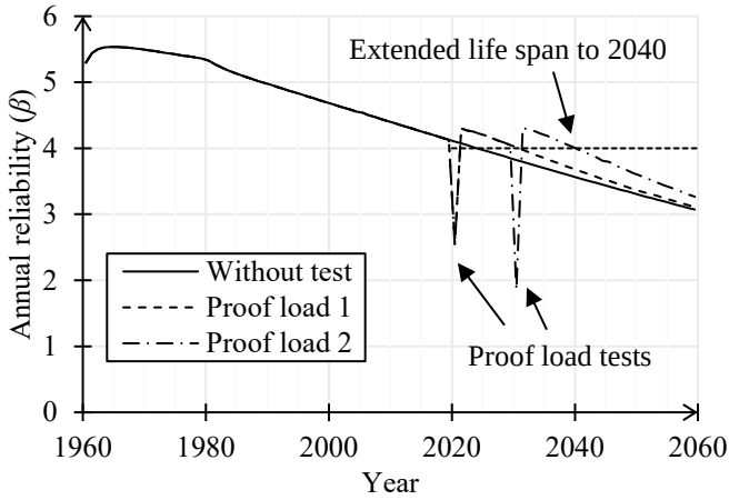
Figure 6: Effect of proof load testing on the annual reliability.
