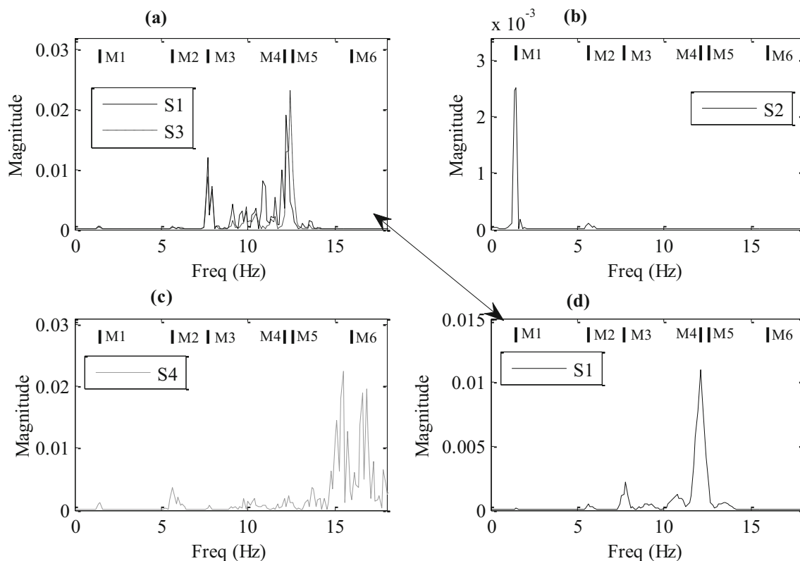
Fig. 8 Frequency content of accelerations signals from bridge sensors due to vehicle passage at 30 \text{ km h}^{-1} over a Class ‘A’ profile. a Frequency content of sensors S1 and S3; b frequency content of
