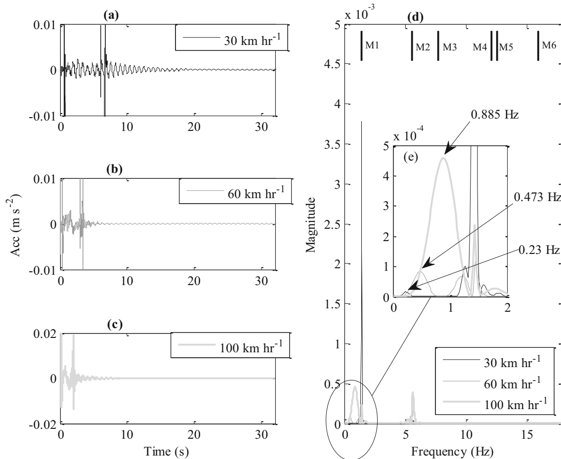
Fig. 10 Effect of vehicle velocity on frequency response of structure—sensor S2. a Acceleration measured due to vehicle traversing at 30 \text{km h}^{-1} + 30 s free; b acceleration measured due to vehicle
