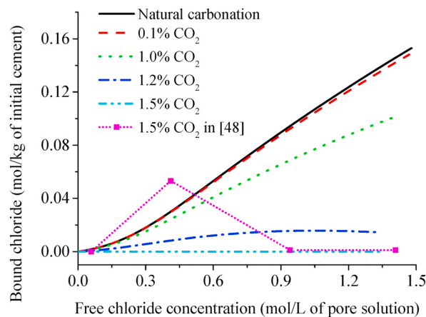
Fig. 7. Predicted chloride binding isotherms (CBIs) in the completely carbonated paste at different \text{CO}_2 concentrations.
