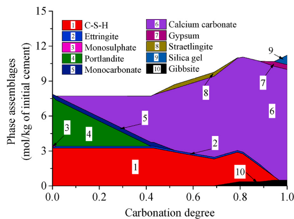
Fig. 8. Phase assemblages in the paste as a function of carbonation degree at 1.5% \text{CO}_2 concentration.
