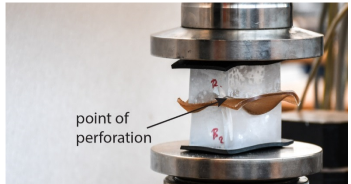
Figure 6: Typical failure at the edge of the assembly caused by the perforation/tearing of the interlayer (specimen 60A 1 )
