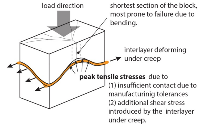
Figure 5: Possible explanation of the cause of failure of the specimens interleaved with PMC770 (70A) and Task16 (80A).
