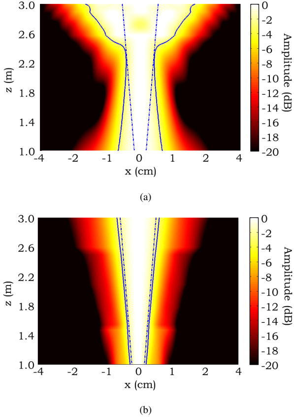
Fig. 7. xz-cut of the field scattered by the quasi-optical system: (a) no refocusing, (b) mechanical refocusing. The dot-dashed and solid lines correspond to the ideal and actual cross-range HPBW, respectively.
