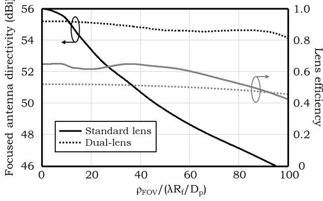
Fig. 2. Performance at 500 GHz as a function of the scanning in the image plane of the standard focusing lens of Sec. II-B and the inversely magnified dual-lens of Sec. II-C. The black and gray curves correspond to the focused antenna directivity and lens efficiency, respectively.
