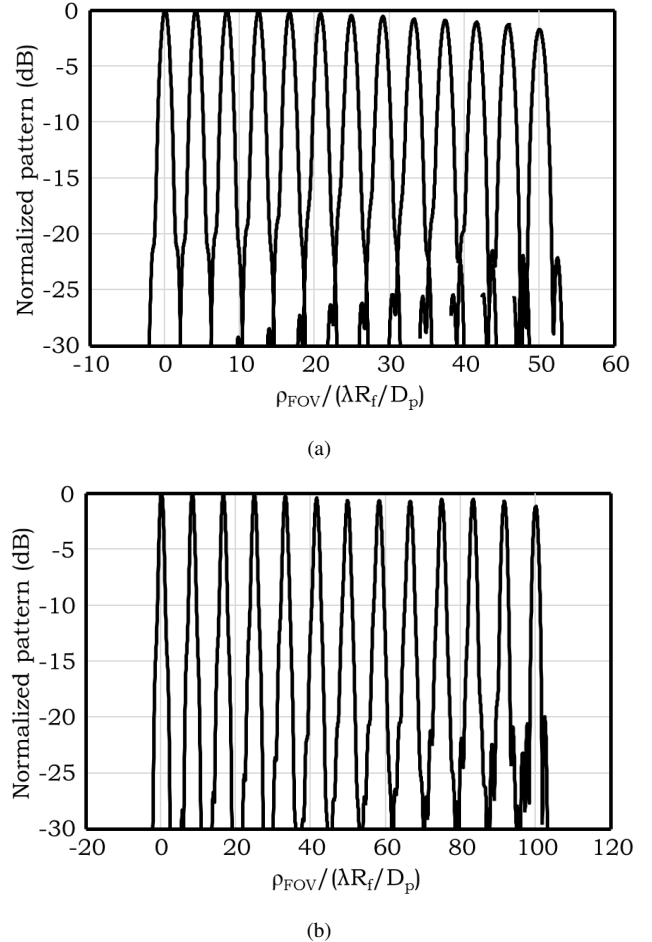
Fig. 4. Normalized patterns in the image plane of the inversely magnified dual-lens system: (a) 250 GHz, (b) 500 GHz.
