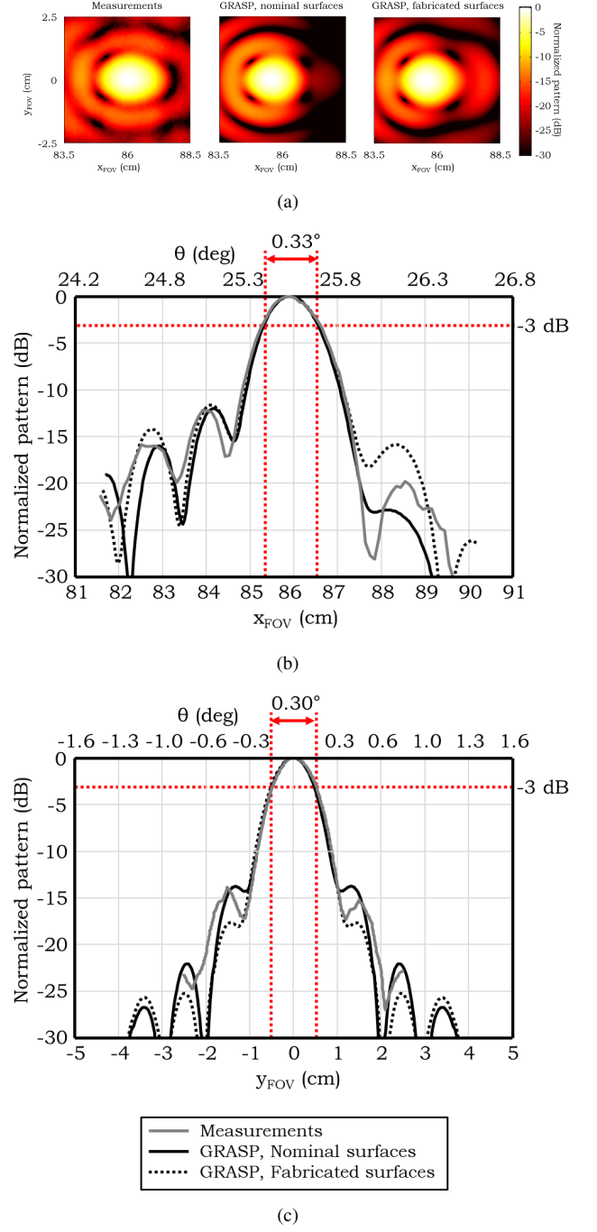
Fig. 10. Measured patterns for 100 HPBW scanning at 500 GHz and R_f = 1.8 m: (a) 2D-pattern in the image plane (b) x-cut, (c) y-cut.
