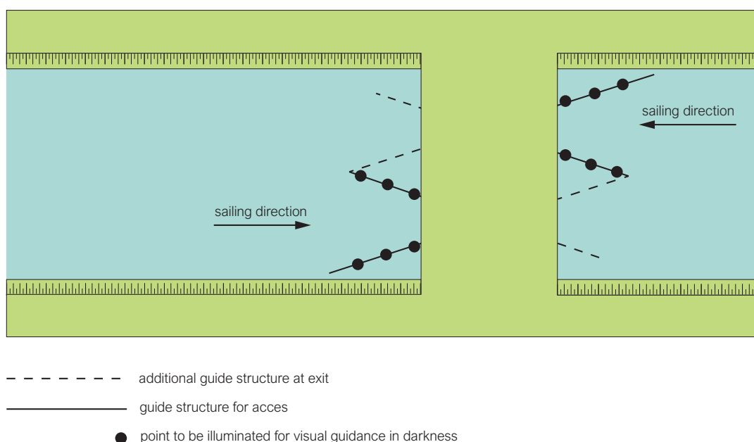
Figure 5.5: Illumination of a bridge passage (reworked from Brolsma et al., 2008, by TU Delft – Ports and Waterways is licenced under CC BY-NC-SA 4.0).
