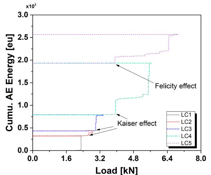
Fig. 10. Cumulative AE energy versus load curve for the five load cycles.
