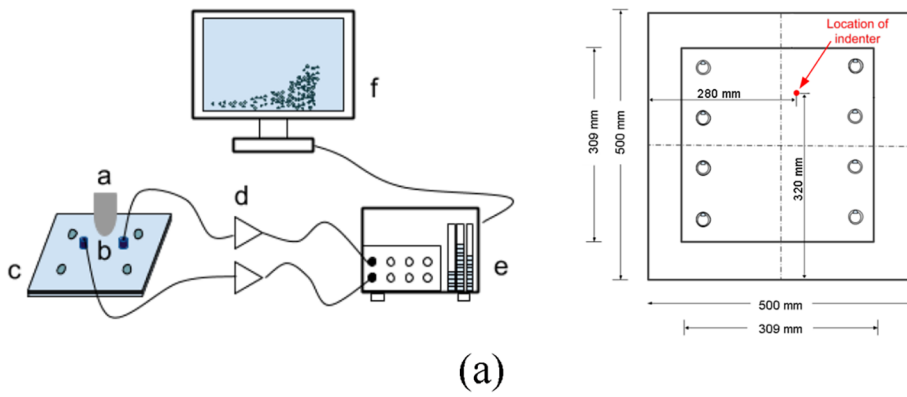
Fig. 4. a) The schematic of impact location and configuration of sequential indentation tests (test apparatus description: (a) indenter, (b) AE sensors, (c) composite panel, (d) preamplifiers with a gain of 34 dB, (e) Vallen AMSY-6 acoustic signal processor, and (f) laptop with Vallen Acquisition and Vallen Visual TM software), and b) the experimental test apparatus for sequential indentation tests.
