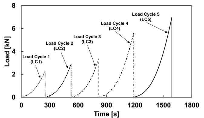
Fig. 3. The sequential increasing indentation load.
