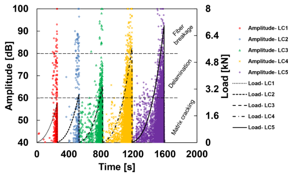
Fig. 7. AE amplitude and load versus time curves for the five load cycles.
