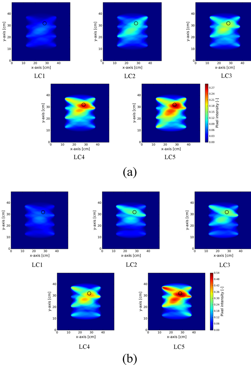
Fig. 13. Image reconstruction for the five load cycles, a) DI_{Pearson} , and b) DI_{Energy} .
