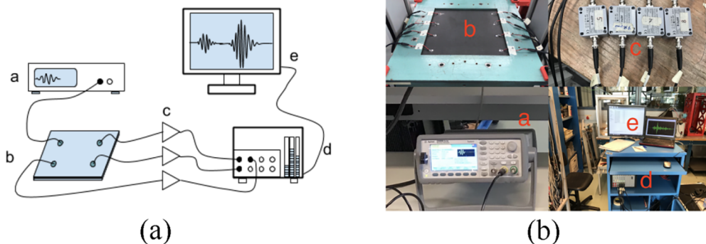
Fig. 2. a) The schematic, and b) the real view of the experimental setup for baseline tests (test apparatus description: (a) Agilent 33500B Series waveform generator, (b) panel with attached sensors, (c) preamplifiers with a gain of 34 dB, (d) Vallen AMSY-6 acoustic signal processor, and (e) laptop with Vallen Acquisition and Vallen Visual TM software).
