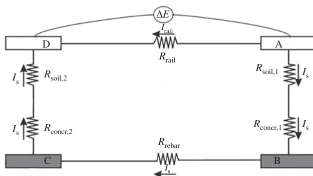
Figure 13: Equivalent electrical circuit to the scenario shown in Figure 5.
