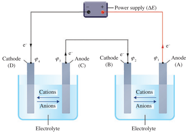
Figure 16: Series of electrolytic cells I and II.
