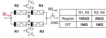
Fig. 9. Modified reference cells.
