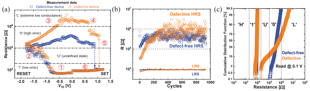
Fig. 4. Comparing defect-free and defective devices. (a) Measured R - V curve in the logarithmic y -axis, (b) Measured R_{\text{RESET}} and R_{\text{SET}} in multiple (936) cycles, (c) Lognormal distributions of R_{\text{RESET}} and R_{\text{SET}} in multiple (936) cycles (read at 0.1 V).
