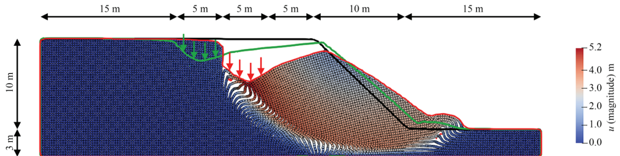
Figure 4 End of a simulation with c_u^i = 50 kPa; MPs and their colour represent the displacement for q = 100 kPa (case 1); PFM edge for q = 100 kPa (case 1) coloured in red; PFM edge for q = 100 kPa (case 2) coloured in green; PFM edge for q = 0 kPa coloured in black.
