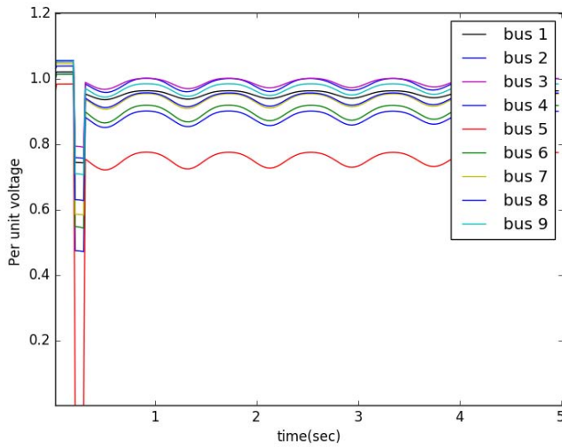
Fig. 5: Bus voltages of IEEE 9-bus system during an FIDVR event
