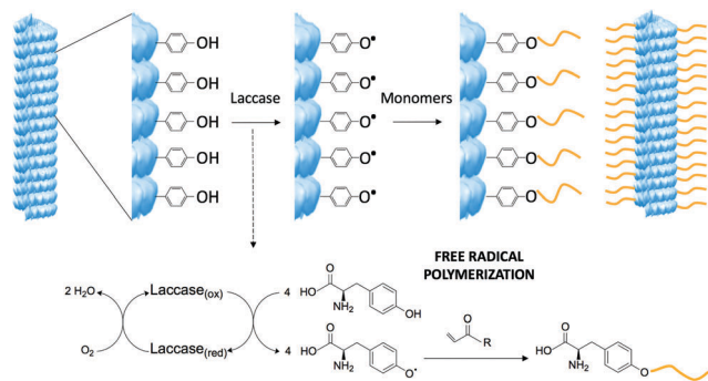
Scheme 1 Modification of the tobacco mosaic virus via laccase induced free-radical oxidation. Laccase oxidizes the exposed tyrosine residues on the viral surface and the phenolic radicals newly formed triggers the functionalization of acrylate monomers. TMV structure created from the RCSB PDB ( www.rcsb.org ) of PDB ID 2OM3. 13
