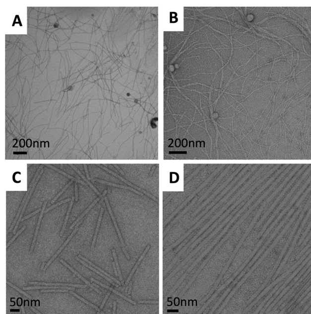
Fig. 1 Transmission electron micrographs of the virus particles. (A) M13 unmodified (B) M13–NIPAM hybrid (C) TMV unmodified and (D) TMV–NIPAM hybrid.
