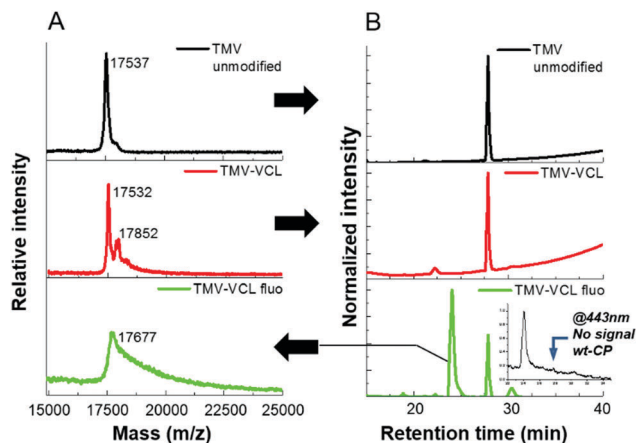
Fig. 2 MALDI-ToF spectra and RPLC elugrams of TMV particles. (A) From the top to the bottom MALDI-ToF spectra of CP derived from TMV unmodified particles, CP derived from TMV-VCL hybrids, CP functionalized fraction isolated through RPLC from TMV-VCL fluorescent hybrids. (B) RPLC elugrams (detection at 254 nm) of CP derived from TMV unmodified particles, CP derived from TMV-VCL hybrids, and CP derived from TMV-VCL fluorescent hybrids. Inset elugram (detection at 443) of TMV-VCL fluorescent hybrids.
