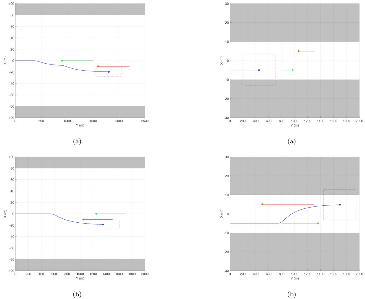
Fig. 4. Head-on scenarios with multiple NSs.
