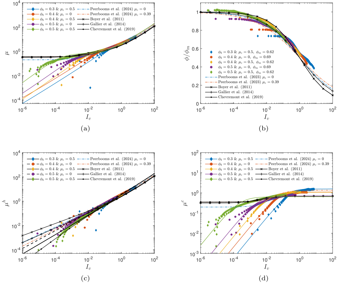
Fig. 19 Local frictional rheology as a function of the viscous number I_v . a Macroscopic friction coefficient \mu . b Normalized solid volume fraction \phi/\phi_m . c Hydrodynamic contribution to the macroscopic friction coefficient, \mu^h , and d contact contribution to the macroscopic friction coefficient, \mu^c . Lines show model descriptions as specified in the legends of the figures
