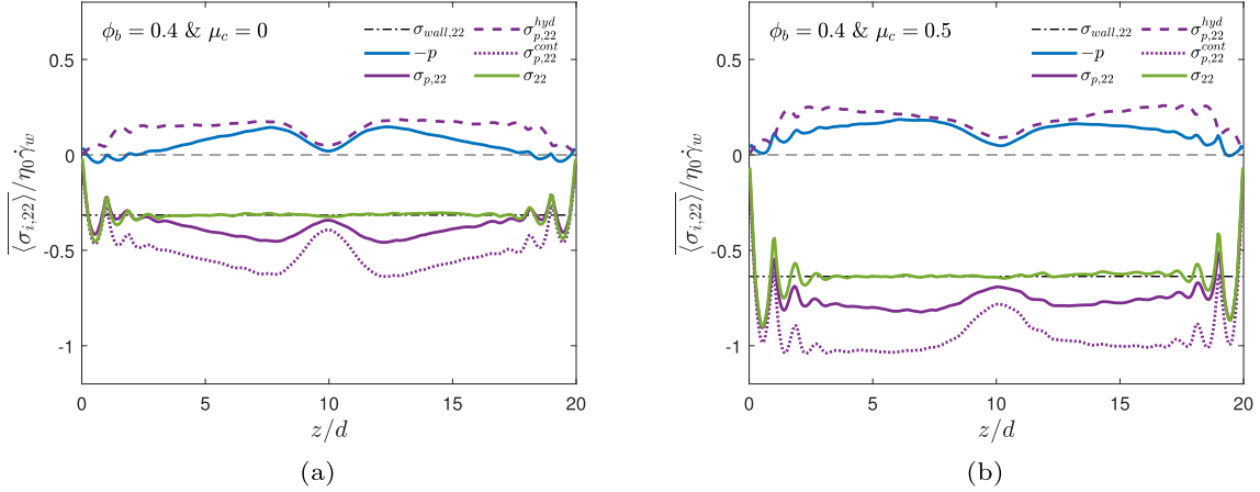
Fig. 16 Steady-state mean superficial wall-normal stress \langle \sigma_{i,22} \rangle as a function of the wall-normal coordinate for \phi_b = 0.4 with \mu_c = 0 (a), and \mu_c = 0.5 (b). Different colors indicate the various stress terms, while the dashed and the dotted lines show the hydrodynamic and the contact contribution to the particle stress, respectively. The black dash-dotted line is the wall-normal stress computed from the average particle/wall contact force per unit wall area
