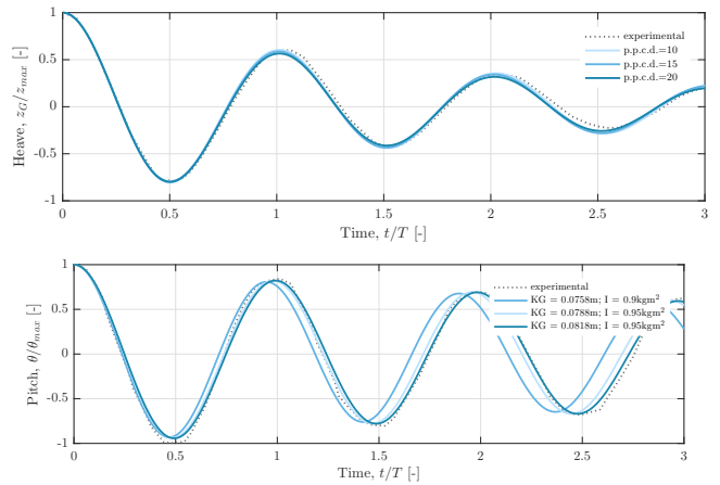
Fig. 3. Decay tests in heave (top) and pitch (bottom). The displacements are normalised by the maximum initial values, 0.076 m and 8.88^\circ , respectively, and the time by the experimental natural periods, which are 1.11 s in heave and 1.17 s in pitch.
