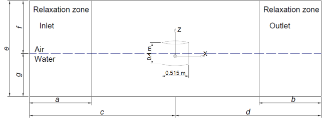
Fig. 2. Numerical domain set-up, with the dimensions indicated with letters in meters, cylinder diameters (D) and wave lengths (w.l.): a = 3 \text{ m} = 5.80 D ; b = 6 \text{ m} = 11.65 D ; c = 9 \text{ m} = 17.50 D ; d = 9 \text{ m} = 17.50 D ; e = 1.8 \text{ m} ; f = g = 0.9 \text{ m} . The width of the domain is 5 m.
