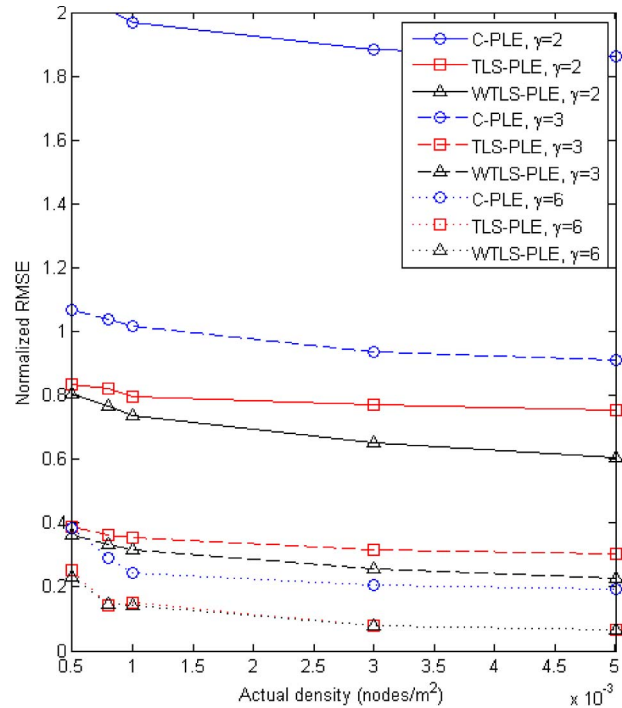
Fig. 9. Performance of three considered estimators with an increasing actual density.
