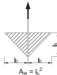
Fig. 3. Effective area of the cone of the mortar joint for shear strength.
