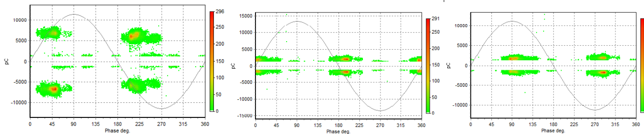
Fig.10. PRPD pattern of the defect measured using Coupling Capacitors.
