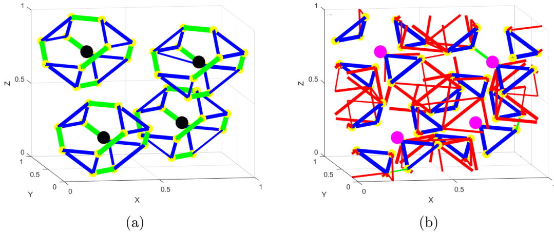
Figure 7: Jump statistics plots from MD-simulations at 450 K of \text{Li}_6\text{PS}_5\text{Cl} with all chloride (a) on 4a (outside the cages) and (b) on 4c (inside the cages). The lines represent the three different types of jumps; green: doublet, blue: intracage, red: intercage, thicker lines represent larger jump rates. The coloured spheres indicate; black: S at 4c, pink: Cl at 4c, yellow: Li-ion sites (48h).
