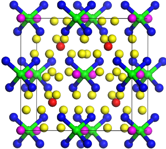
Figure 1: Crystal structure of HT- \text{Li}_7\text{PS}_6 15 . Colours correspond to; yellow: Li-sites (48h), green: phosphorus, blue: bonded sulphur, pink: 4a-sites, red: 4c-sites
