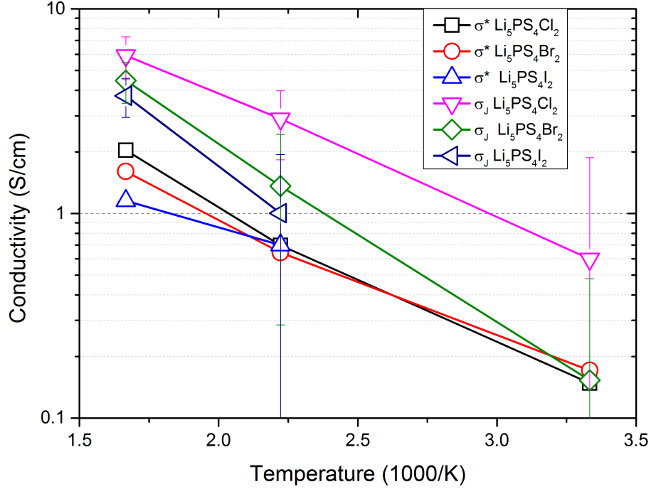
Figure 9: Arrhenius plot of the conductivities of \text{Li}_5\text{PS}_4\text{X}_2 compounds from MD-simulations based on the intercalation jump frequency, \sigma_J , and the MSD, \sigma^* .
