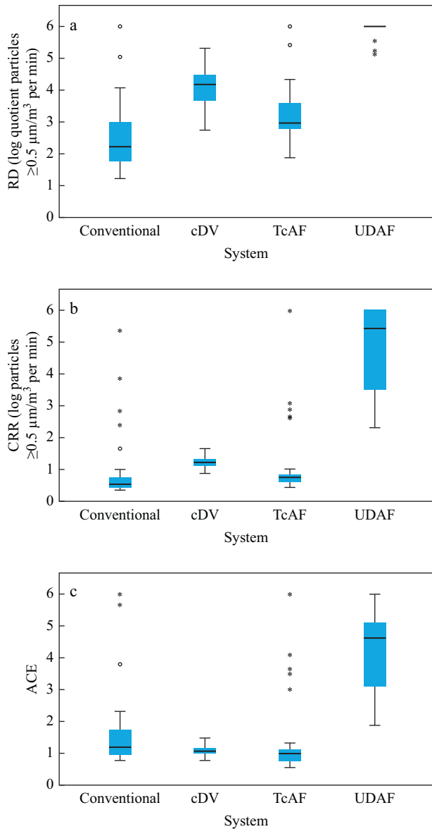
Figure 7. (a) Recovery degree over a 10-min period ( \text{RD}_{10} ), (b) cleanliness recovery rate (CRR) (c) and air change effectiveness (ACE) for conventional ventilation (CV), controlled dilation ventilation (cDV), temperature-controlled airflow (TcAF) and unidirectional airflow (UDAF) systems in area A. The CV and TcAF systems were comparable in terms of \text{RD}_{10} ( P=0.09 ) and CRR ( P=0.60 ). The TcAF and cDV systems ( P=0.62 ) and CV and cDV systems ( P=0.51 ) were comparable in terms of ACE. All other comparisons between systems showed significantly different \text{RD}_{10} , CRR and ACE ( P<0.01 ).
