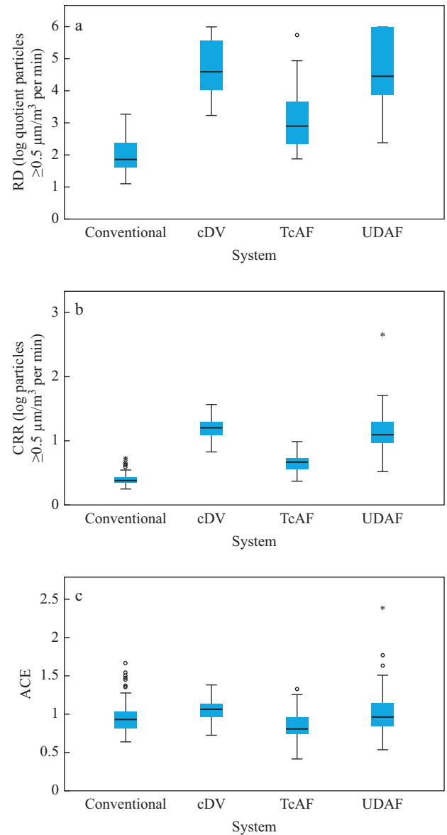
Figure 8. (a) Recovery degree over a 10-min period ( \text{RD}_{10} ), (b) cleanliness recovery rate (CRR) (c) and air change effectiveness (ACE) for conventional ventilation (CV), controlled dilation ventilation (cDV), temperature-controlled airflow (TcAF) and unidirectional airflow (UDAF) systems in area B. The cDV and UDAF systems were comparable in terms of \text{RD}_{10} ( P=0.73 ) and CRR ( P=0.05 ). The UDAF and CV systems were comparable in terms of ACE ( P=1.00 ). All other comparisons between systems showed a significantly different \text{RD}_{10} , CRR and ACE ( P<0.01 ).
