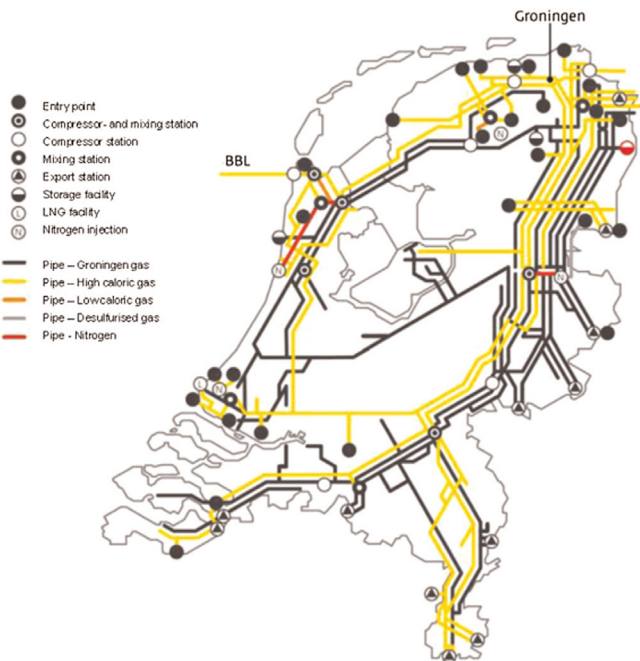
Fig. 3. Gas Transmission in the Netherlands.
