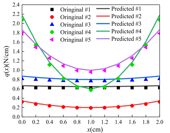
Fig. 8. Comparison between the predicted solutions and the analytical solutions of mechanical loads.
