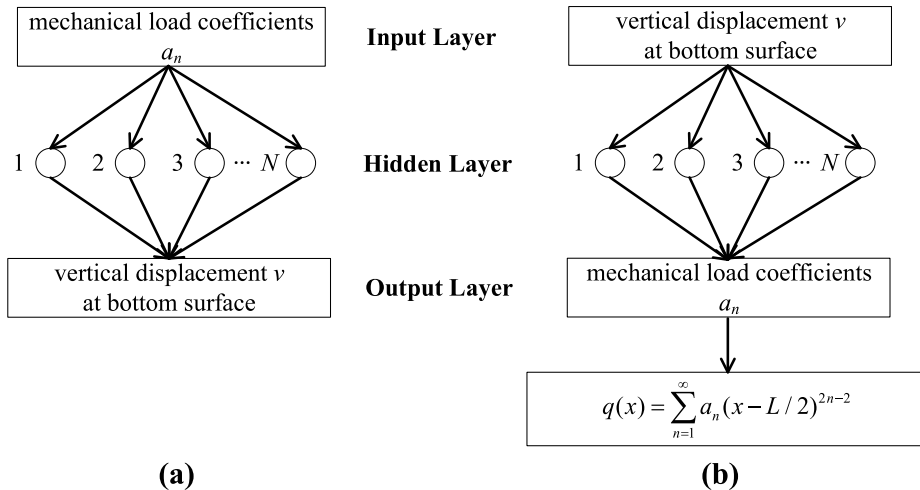
Fig. 2. The structure of the BP neural network: (a) predict the deformation based on the mechanical load; (b) inverse the mechanical load based on the deformation.
