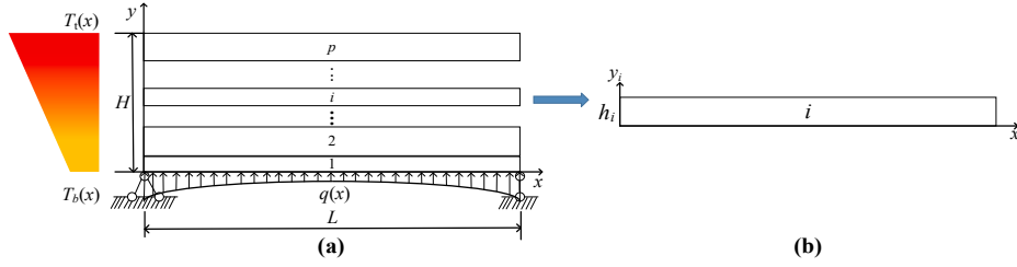
Fig. 1. Two-dimensional multi-layer simply supported beam under combined thermo-mechanical load.
