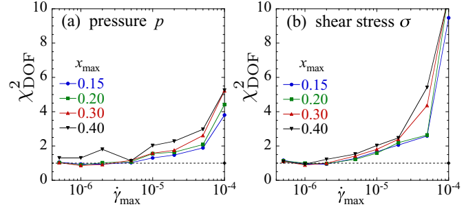
FIG. 4. \chi^2 per degree of freedom \chi_{\text{DOF}}^2 of our fits of (a) pressure p and (b) shear stress \sigma to the scaling form of Eq. (11) without corrections to scaling (i.e., taking w = 0 ), as a function of the upper limit \dot{\gamma}_{\text{max}} of data used in the fit. We show results for several different values of x_{\text{max}} , where only data with |x| = |\delta\phi|/\dot{\gamma}^{1/z\nu} \leq x_{\text{max}} are used in the fit. Data are restricted to the range 0.838 \leq \phi \leq 0.846 .
