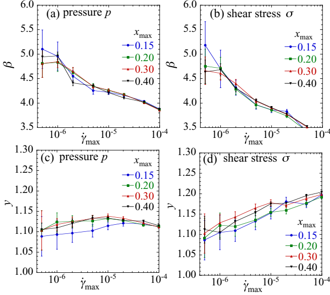
FIG. 7. Exponents \beta = (2 - q)z\nu and \gamma = qz\nu obtained from the fit parameters of Fig. 6 for pressure p (left column) and shear stress \sigma (right column) vs the strain rate cutoff \dot{\gamma}_{\max} . We show results for different values of the additional cutoff x_{\max} , where only data with |x| = |\delta\phi|/\dot{\gamma}^{1/z\nu} \leq x_{\max} are used in the fit. Results are from fits to the scaling form of Eq. (11) without corrections to scaling (i.e., taking w = 0 ).
