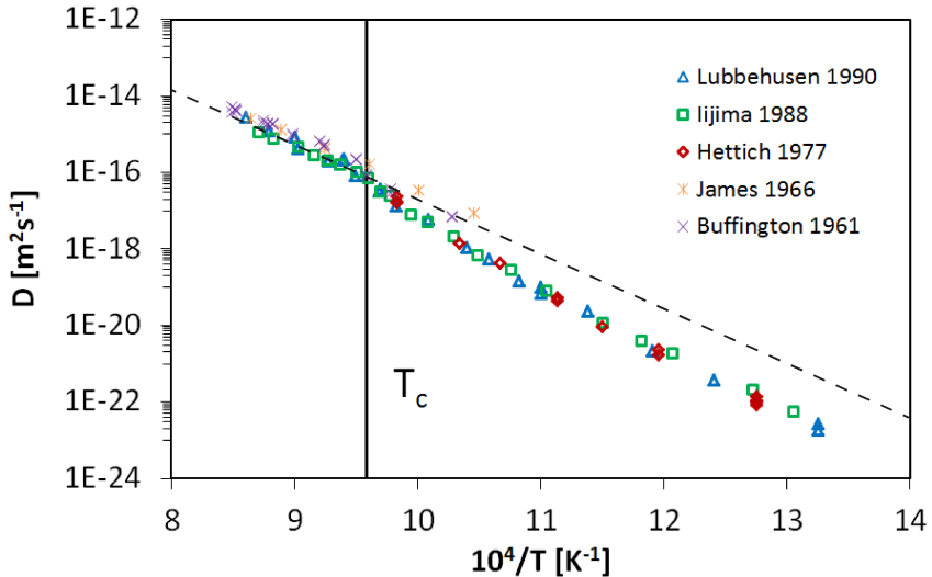
Figure 3.1: Experimental data of iron self-diffusivity as a function of the inverse temperature [1–5]. The Curie temperature is indicated as T_C , and the dashed line is an extrapolation of Arrhenius behaviour of the paramagnetic state above T_C .
