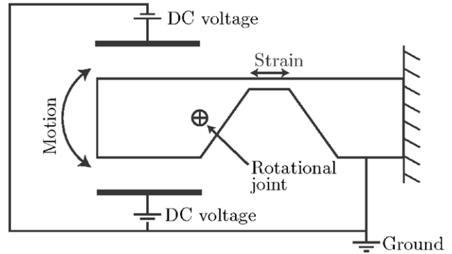
Figure 32. Schematic of device [84].
