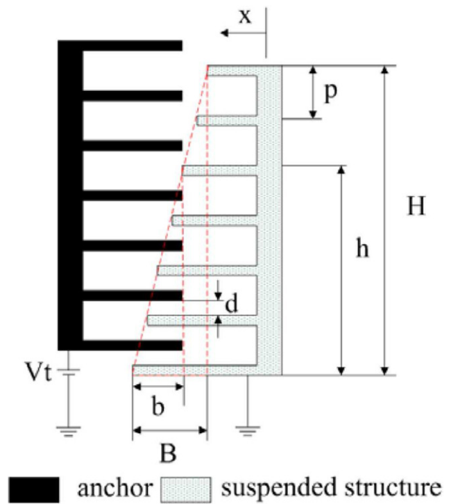
Figure 12. Tuning-comb of the tunable resonator. Reprinted from [17], used under the terms of the creative commons attribution 4.0 license.
