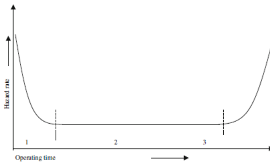
Figure 2.1: Bath-tub curve [20]
