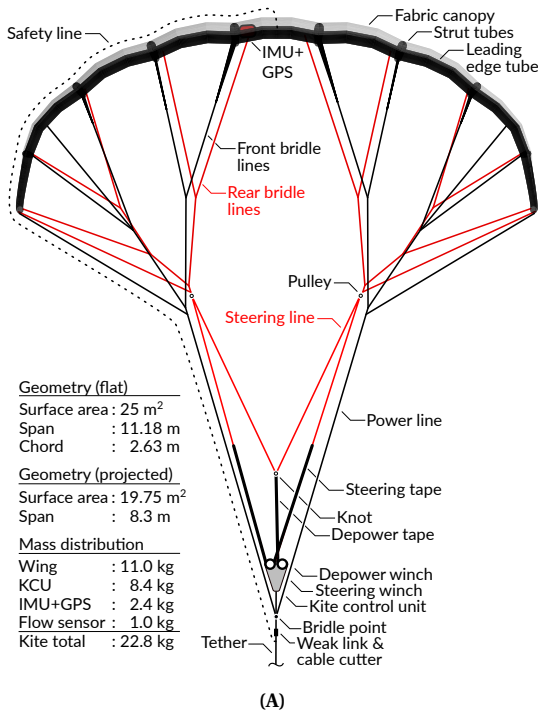
Figure 3.2: A, Front view of the leading-edge inflatable (LEI) V3 kite [60]; B, Photo of the V5.40 with 40 m 2 wing surface area (courtesy of Kitepower B.V.).
