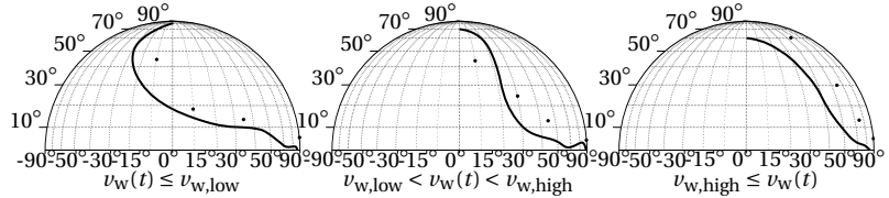
Figure 3.5: Observed landing paths of the kite on the flattened spherical coordinate plane for different wind speed ranges [41].
