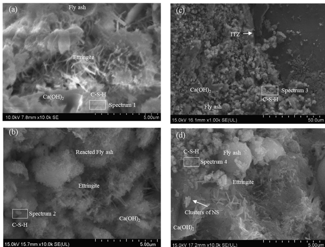
Fig. 4. SEM images of mortar with (a) 0%, (b) 3%, (c) 3% (with ITZ) and (d) 5% of NS.
