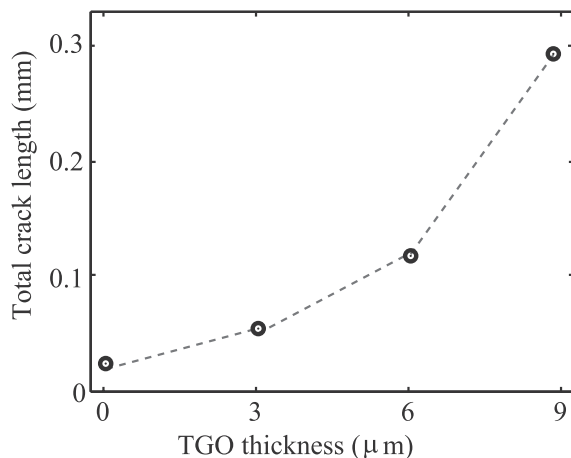
Fig. 12. Variation of total crack length for different TGO thickness 0, 3, 6 and 9\text{ }\mu\text{m} with 15% random microstructural pores.
