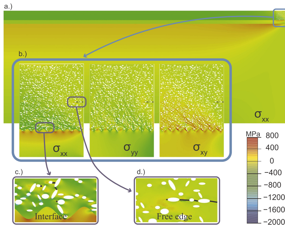
Fig. 8. Stress distribution in TBC with realistically represented microstructural pores at T = 30^\circ\text{C} . a.) Stress variations ( \sigma_{xx} ) in the concurrent multiscale TBC model b.) Stress distribution in the TBC computational cell with explicitly modelled pores. c.) Mixed mode Cracking of interior TC layer close to BC due to pores and thermal mismatch stress. d.) Mode I cracking at the edge of the TC layer due to free edge effect.
