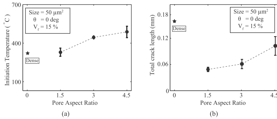
Fig. 6. Variation of (a) crack initiation temperature and (b) total crack length for different pore aspect ratio 0 (dense), 1.5, 3 and 4.5 with the fixed pore size of 50 \mu\text{m}^2 , orientation of 0^\circ and volume fraction of 15%.
