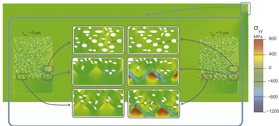
Fig. 11. Stress distribution in TBC with random microstructural pores at T = 30\text{ }^{\circ}\text{C} for TGO thickness of 0\text{ }\mu\text{m} and 9\text{ }\mu\text{m} .
