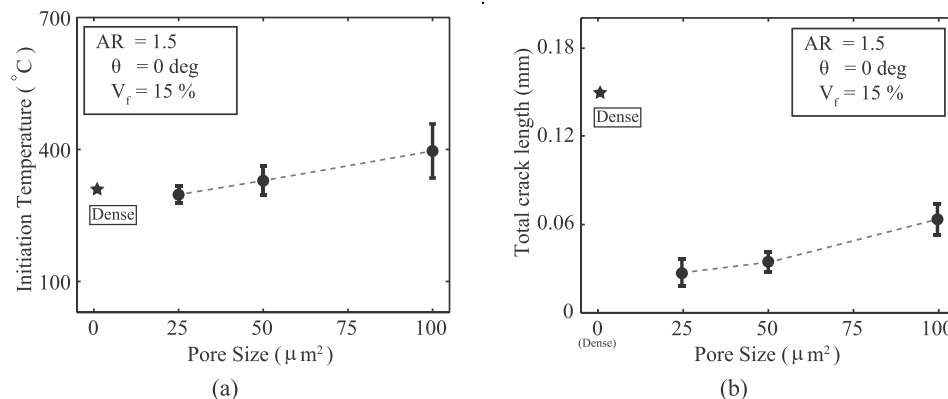
Fig. 5. Variation of (a) crack initiation temperature and (b) total crack length for different pore size 0 (dense), 25, 50 and 100 μm² with the fixed pore aspect ratio of 1.5, orientation of 0 deg and volume fraction of 15%.
