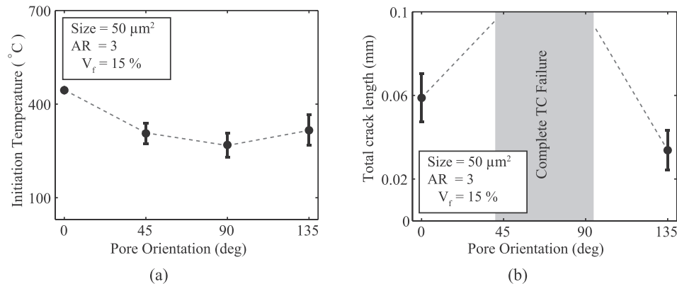
Fig. 7. Variation of (a) crack initiation temperature and (b) total crack length for different pore orientation 0, 45, 90 and 135 deg with the fixed pore size of 50 \mu\text{m}^2 , aspect ratio of 3 and volume fraction of 15%.
