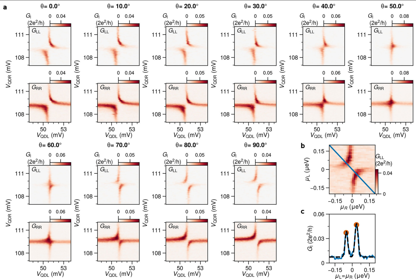
Extended Data Fig. 3 | Extended dataset of Fig. 2. a , CSDs measured at various magnetic field angles \theta between 0° and 90°, used to extract the data shown in Fig. 2d. b , Example of the extraction process. For each obtained CSD, V_{QDL} and V_{QDR} are converted to energies \mu_L and \mu_R using lever arms obtained in
