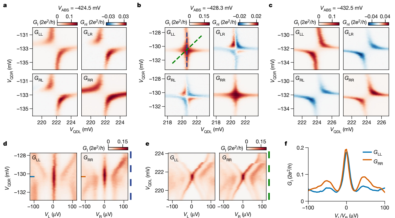
Fig. 3 | Electrostatically tuning to the Majorana sweet spot. a–c , CSDs taken at three different applied voltages V_{\text{ABS}} in device A. The system is smoothly tuned from the \Gamma_o > \Gamma_e regime in a to the \Gamma_o < \Gamma_e regime in c . In between, the \Gamma_o = \Gamma_e condition is satisfied ( b ). A more extensive range is highlighted in Extended Data Fig. 6. d , Tunnelling spectroscopy measurements at the sweet spot.
