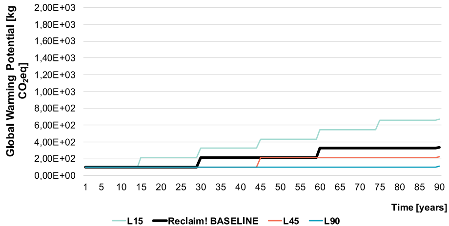
Figure A.IIc. LCA Sensitivity analysis on the L_{\text{technical}} and L_{\text{functional}} for the Reclaim! façade (GWP allocated over 90 years)
