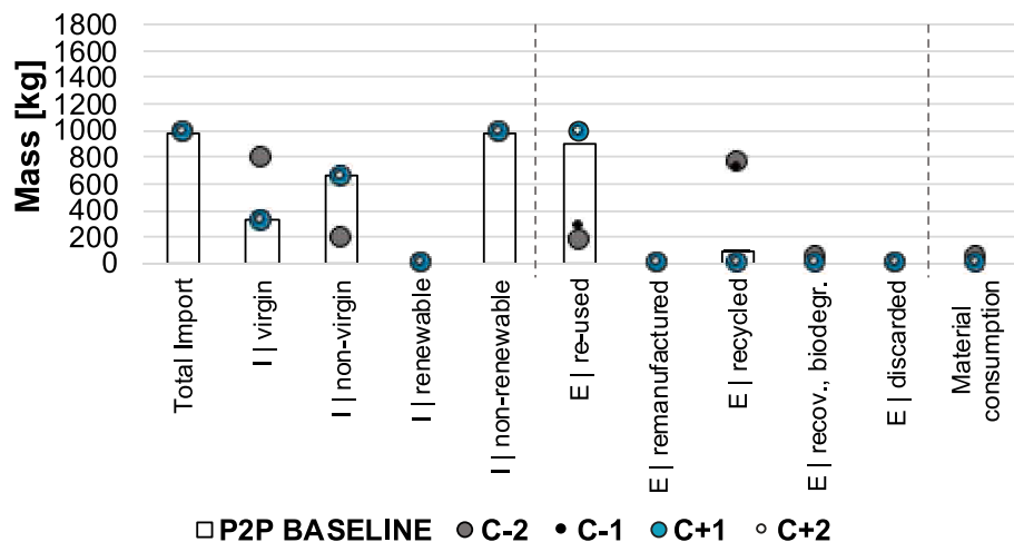
Figure A.G2d. MFA Sensitivity analysis on the number of cycles for the P2P façade (material flows over 90 years)
