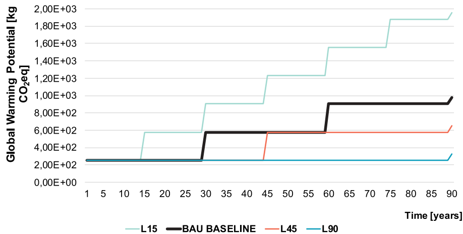
Figure A.IIa. LCA Sensitivity analysis on the L_{\text{technical}} and L_{\text{functional}} for the BAU façade (GWP allocated over 90 years)
