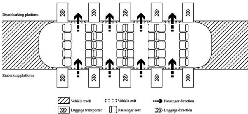
Fig. 2. Concept sketch of the new (dis)embarking solution (top view of hyperloop vehicle on platform).
