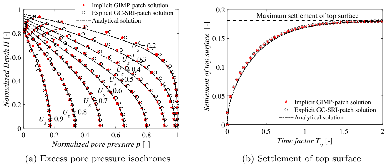
Fig. 9 Comparison between implicit GIMP-patch, explicit GC-SRI-patch and analytical consolidation solutions – large deformation analysis
