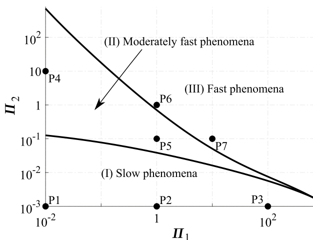
Fig. 6 \Pi_1 – \Pi_2 pairs considered in the implicit GIMP-patch simulation of dynamic consolidation – cf. [38]
