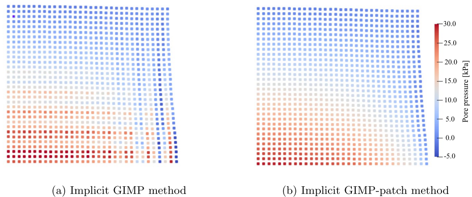
Fig. 12 Excess pore pressure distributions at t = 0.18 s with implicit GIMP and GIMP-patch methods
