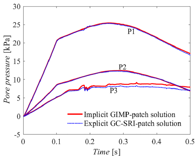
Fig. 14 Time evolution of the excess pore pressure at three different locations (points P1, P2, P3 in Figure 11) obtained for a 2D slumping block using the implicit GIMP-patch method and the explicit GC-SRI-patch method
