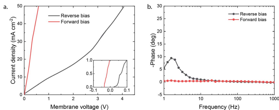
Fig. 3 (a) Linear sweep potentiometry at 0.5 mA \text{s}^{-1} in 1 M NaCl (corrected for electrolyte losses) with positive membrane potential indicating reverse bias and negative forward bias; values at 25 mA \text{cm}^{-2} are 2.74 V (reverse) and 0.41 V (forward). (b) Galvanostatic impedance at 25 mA \text{cm}^{-2} with 6.4 mA \text{cm}^{-2} amplitude.
