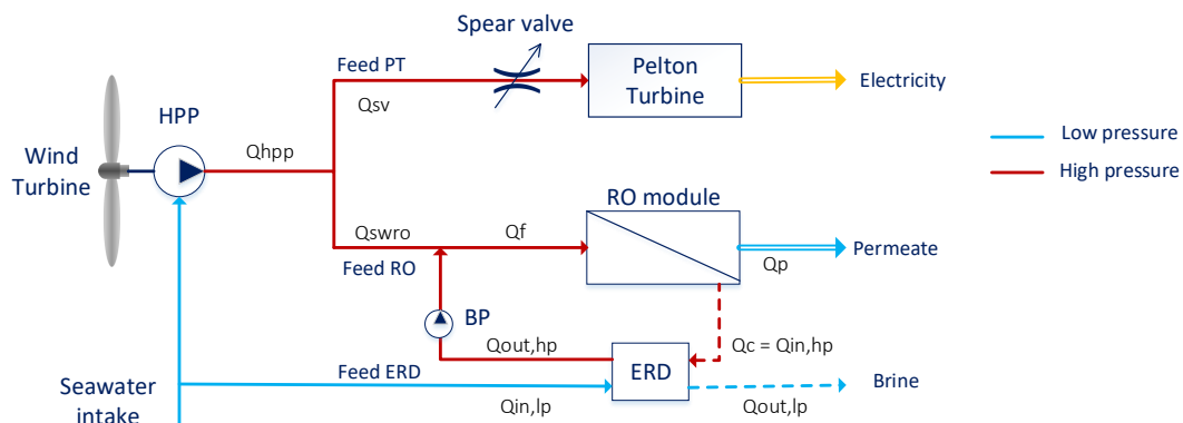
Figure 2: Schematic of the system showing the flow rates in the main points of interest. Solid lines represent seawater, the dashed lines represent the brine and the double lines represent permeate (in blue) and electricity (in yellow)
