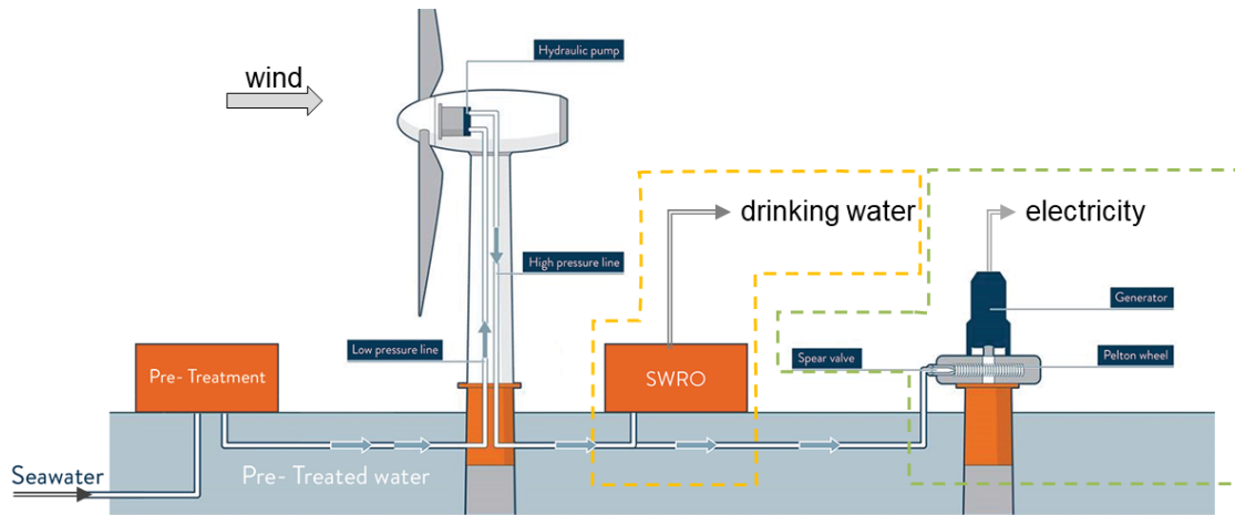
Figure 1: Schematic showing the main components of the wind driven seawater reverse osmosis (SWRO) system. Courtesy of DOT B.V.
