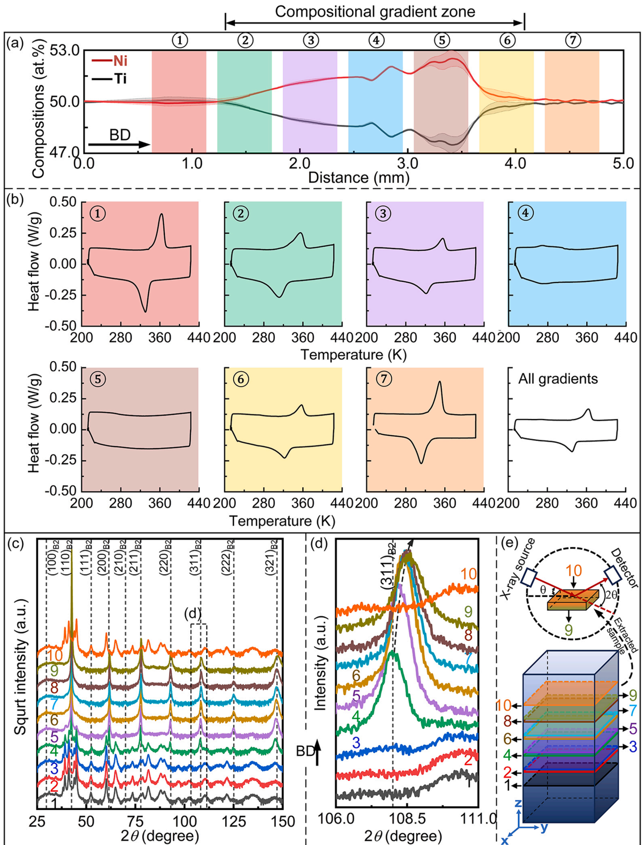
Fig. 2. (a) EDS line scans of Ni and Ti along the building direction. (b) DSC curves of extracted samples from zones with various Ni contents (the corresponding gradient zone was marked in the (a)). (c) XRD patterns along the building direction in the FG zone and the corresponding (d) enlarged (311)_{B_2} peaks. BD is the building direction. (e) Schematic of extracted samples for XRD measurements.
