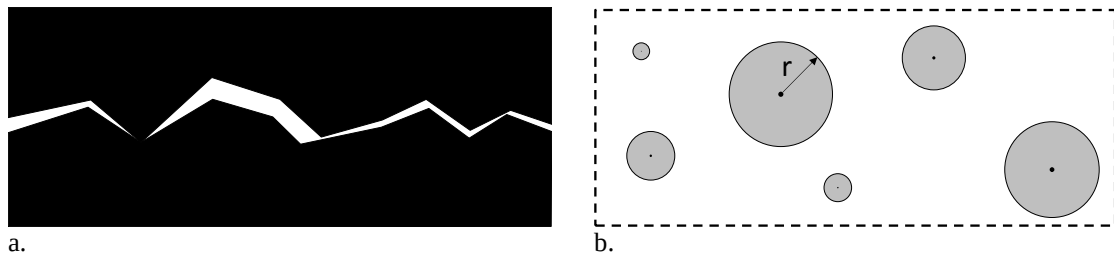
Figure 1 a. Side view of immersing contact points between two surfaces approaching. b. Top view of increasing contact area; area in contact is shown in grey, nucleating from the center point and growing radially indicated by the arrow (r).
