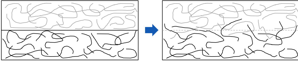
Figure 2. Two pieces of bitumen will adhere to each other as a consequence of the sticky nature of bitumen. Over time, due to molecular motion bitumen molecules will “cross” the interface of two surfaces in contact, resulting in a gradual disappearance of the interface.
