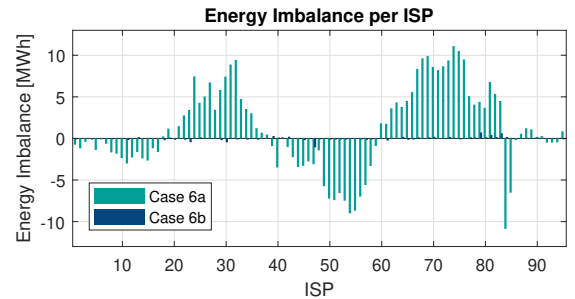
Figure 6. a) Wind Imbalance throughout the simulation for Case 6a & 6b. b) Energy imbalance comparison per ISP.
